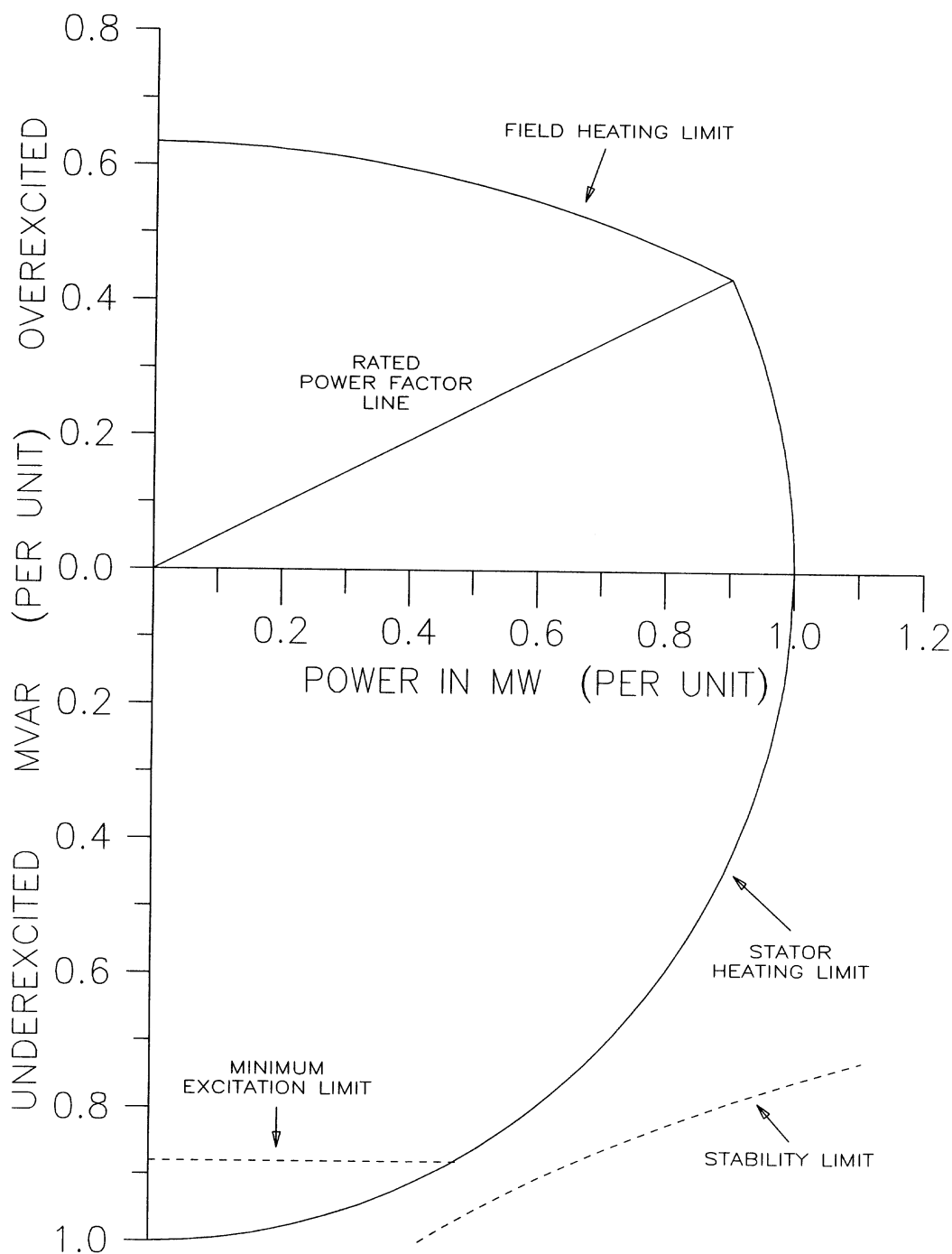
Figure 5—Typical hydro-generator capability curve (0.9 power factor, rated voltage)
